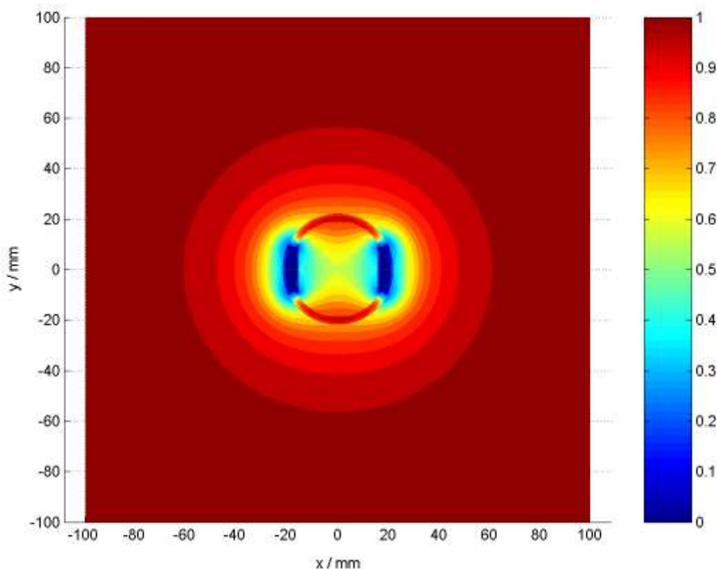
Figure 1: Electric field distribution of the TRIME probe and approximate measuring volume.
