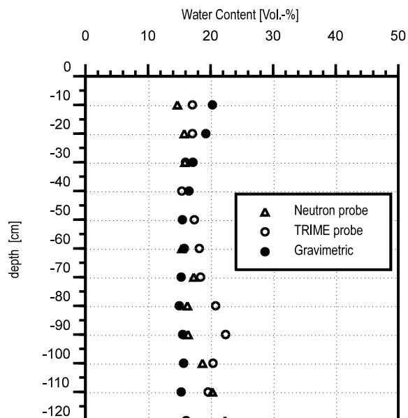
Figure 3: Comparison of neutron probe, TRIME-T3 and gravimetric method for water content determinations in a loess soil.
