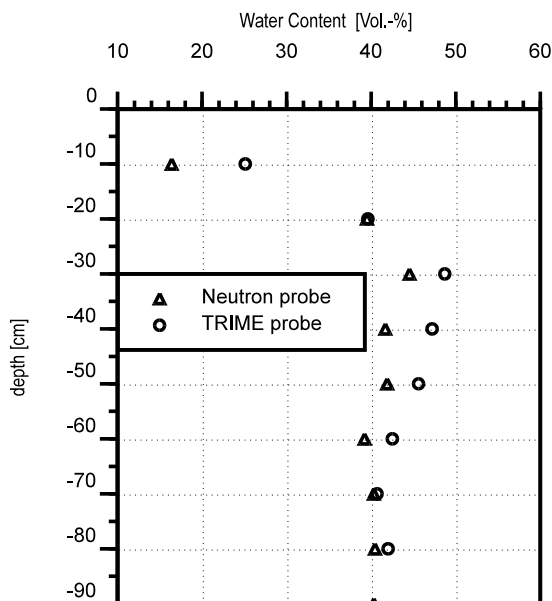
Figure 4 : Comparison of neutron probe and TRIME-T3 for water content determinations in illitic clay.
